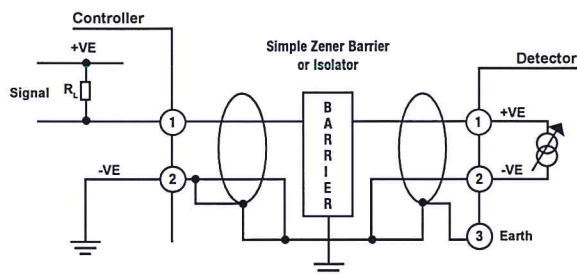
Single Barrier Schematic
