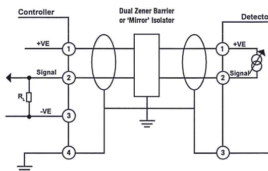
Dual Barrier Schematic
